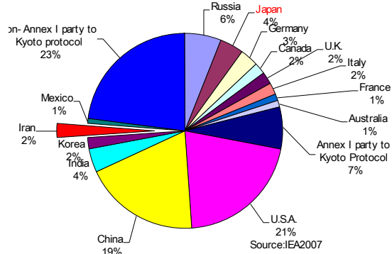
CO2 Emissions from fuel combustion 1971- 2005
